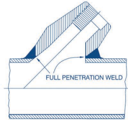
SOCKET-WELD
